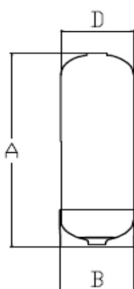
12"-16" TOP OPENING
